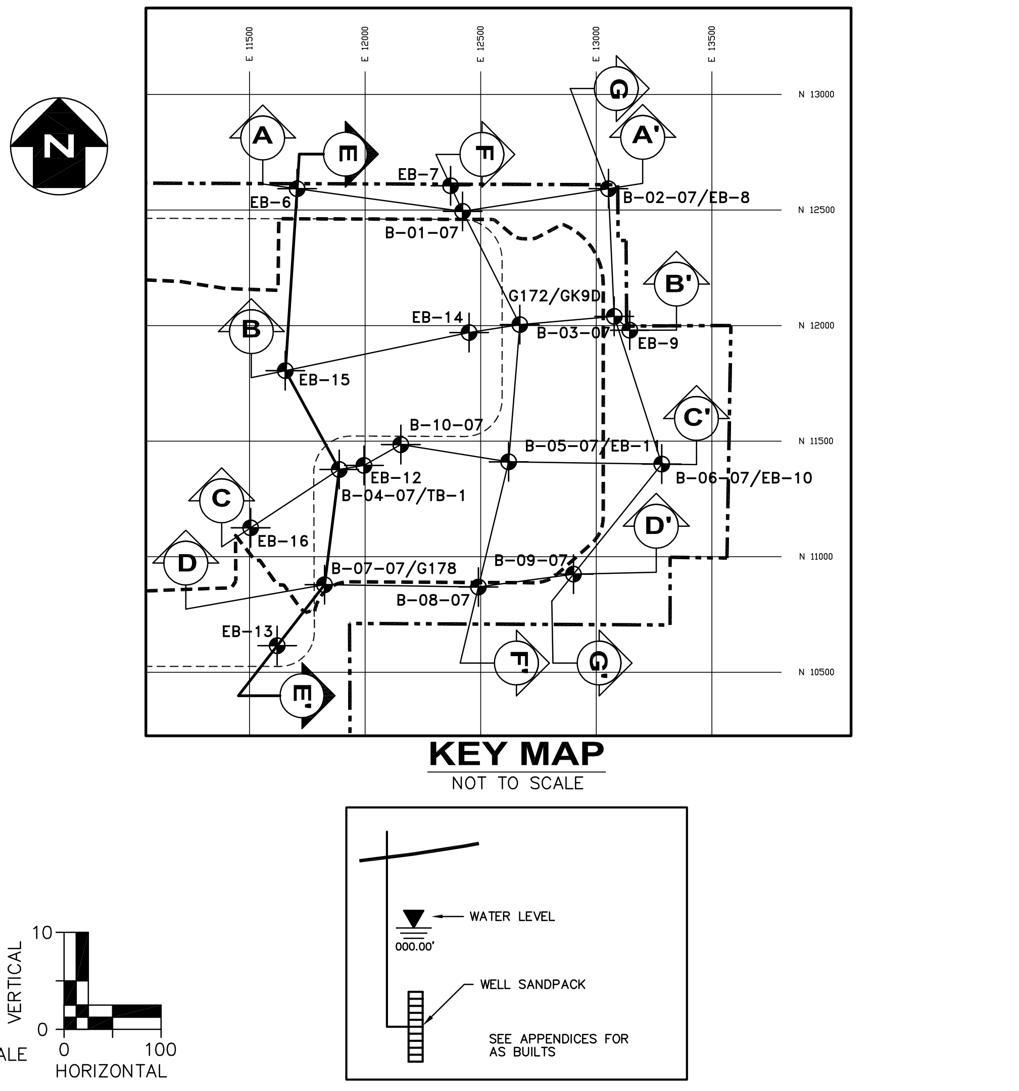
MONITORING WELL/PIEZOMETER SCHEMATIC
