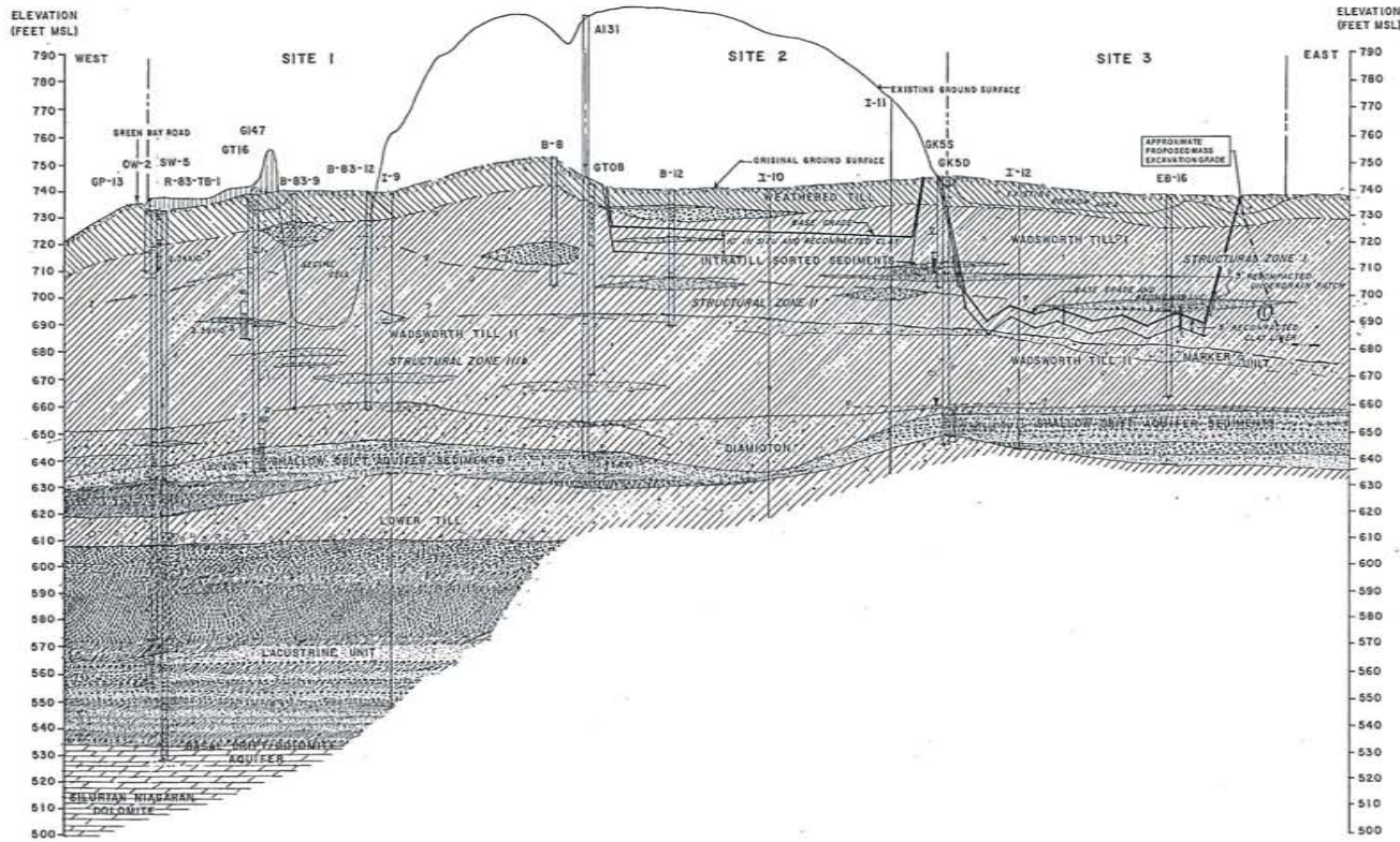
CROSS SECTION F - F'
